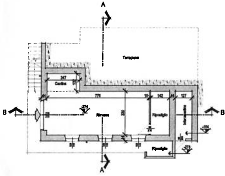
Pianta piano seminterrato Scale 1:100
